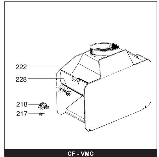
CF - VMC
